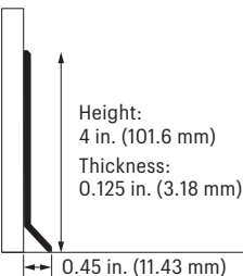
Coved Wall Base
