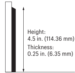
Sculptured Wall Base
