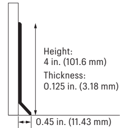
Coved Wall Base
