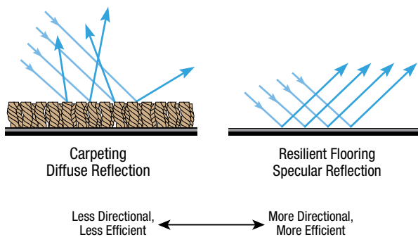
Figure 1: Directionability of Light Reflection
