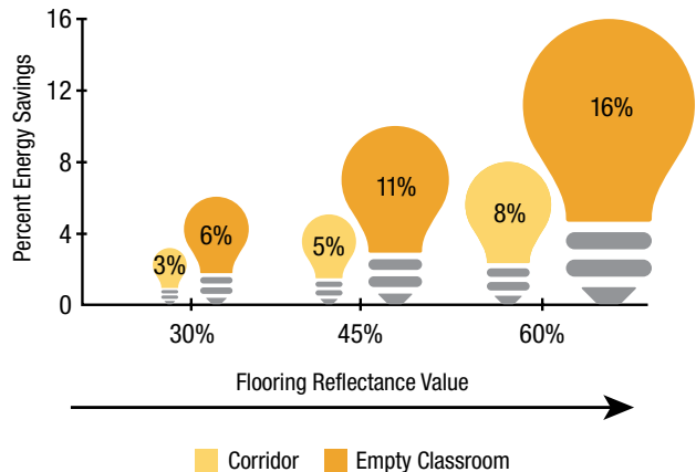
Figure 2: Percent Energy Savings Relative to 10% Floor Reflectance for a Corridor or in an Empty Classroom*
